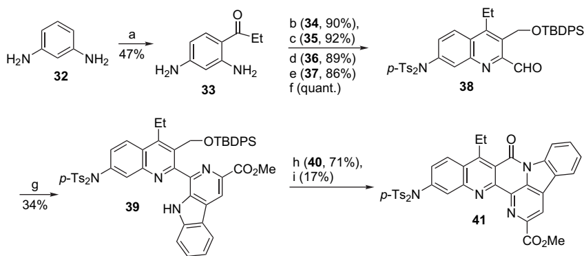
Scheme 4. (a) EtCN, BCl 3 , AlCl 3 , C 2 H 4 Cl 2 ; (b) Me–CO–CH 2 –CO 2 Me, MeOH, H 2 SO 4 ; (c) NaH, THF, Ts 2 O; (d) DIBAL-H, CH 2 Cl 2 , –78 °C; (e) t -BuPh 2 SiCl, DMF, imidazole; (f) SeO 2 , dioxane; (g) tryptophan methyl ester, p -xylene; (h) n -Bu 4 NF, THF; (i) DMP, NMP, pyridine.
